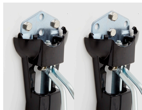
Bolt positions for masonry
